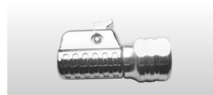
CY-127 Tyre inflation nozzle Product: Material is zinc alloy, with rotating function, self-locking function, connecting port is NPT1/4, G1/4.
